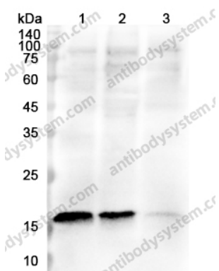
Western blot
