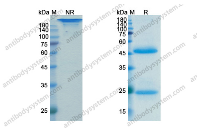
SDS PAGE for Lokivetmab
