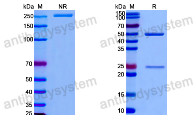
SDS PAGE for G-quadruplex DNA Antibody (8H2)
