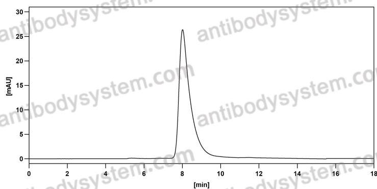
SEC-HPLC
