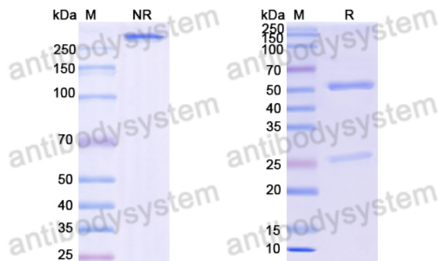
SDS PAGE for DNA Antibody (T24-9)
