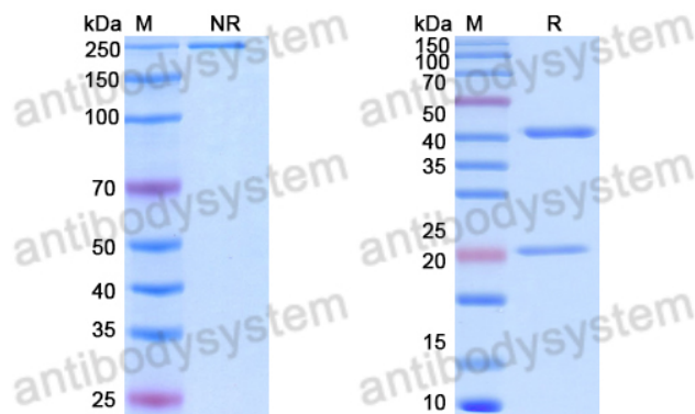
SDS PAGE for DNA Antibody (MRL-22)
