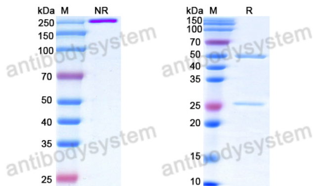
SDS PAGE for DNA Antibody (165.54)
