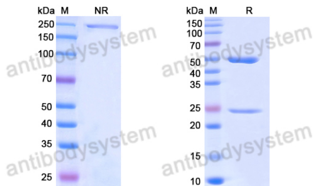
SDS PAGE for DNA Antibody (111.52)
