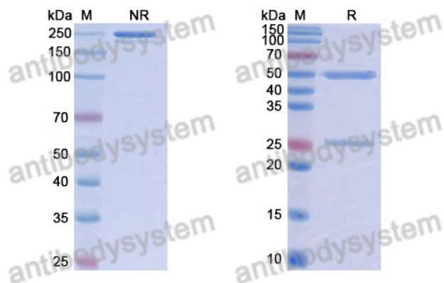
SDS PAGE for DNA Antibody (D23)
