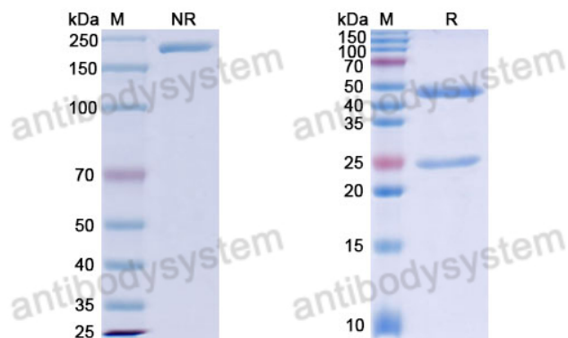
SDS PAGE for DNA Antibody (111.49)
