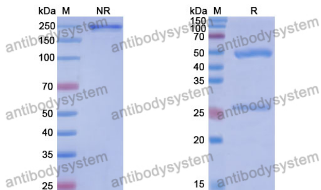
SDS PAGE for DNA Antibody (202.135)
