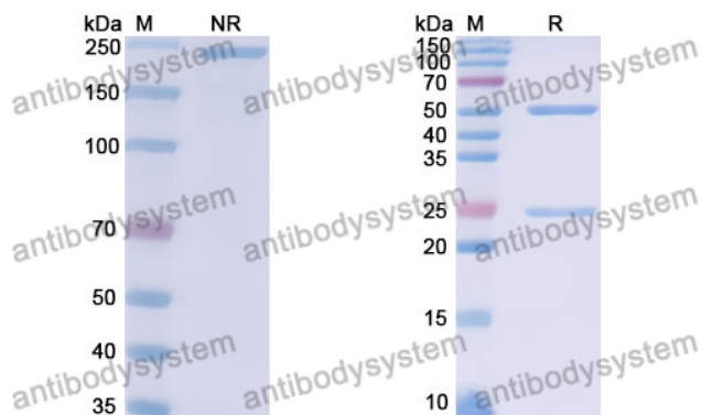
SDS PAGE for DNA Antibody (202s.38)
