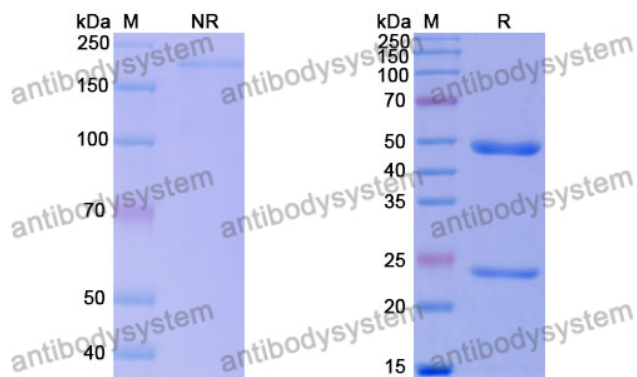
SDS PAGE for DNA Antibody (17s.93m)
