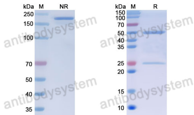
SDS PAGE for DNA Antibody (165.41)
