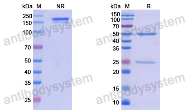
SDS PAGE for DNA Antibody (165.34)
