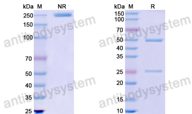
SDS PAGE for DNA Antibody (17s.74)
