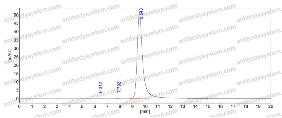
SEC-HPLC
