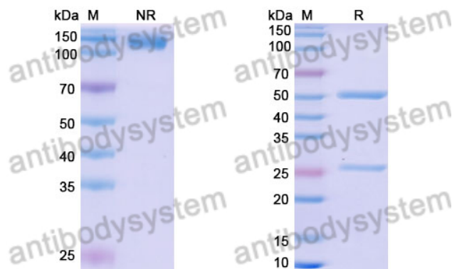
SDS PAGE for Anivovetmab
