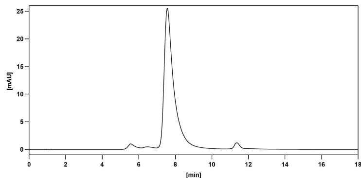
SEC-HPLC
