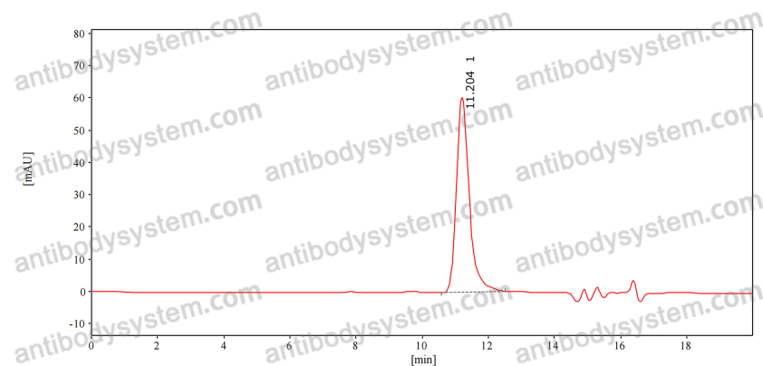
SEC-HPLC
