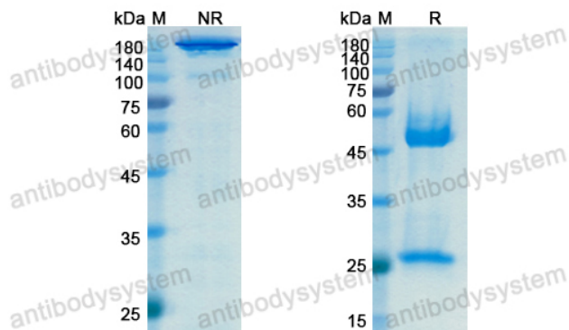
SDS PAGE for STRO-001
