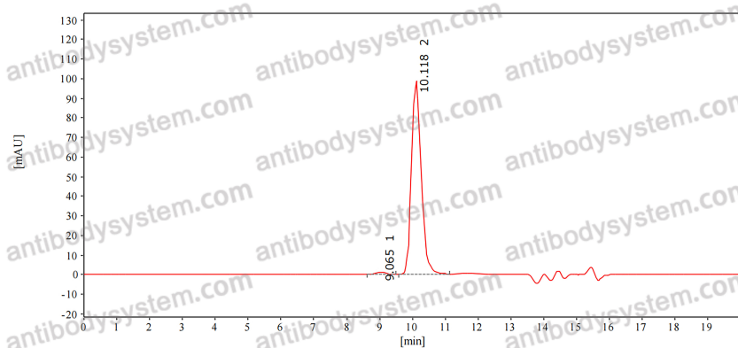
SEC-HPLC
