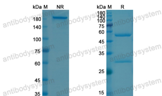
SDS PAGE for Garivulimab
