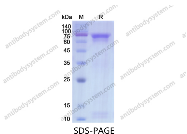
SDS PAGE for recombinant Chlamydia psittaci dnaK / HSP70
