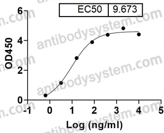
Casirivimab binds with SARS-CoV-2 S - Trimer (WT) protein
