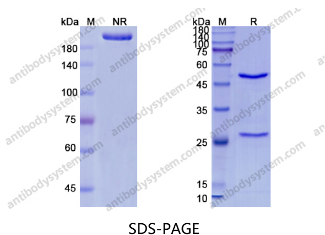
SDS PAGE for Urtoxazumab
