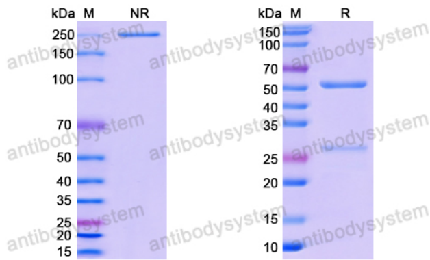
SDS PAGE for Anti-SARS2 RBD Antibody(R3P2-G1)
