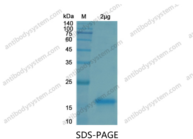
SDS PAGE for recombinant SARS-CoV-2 NSP9
