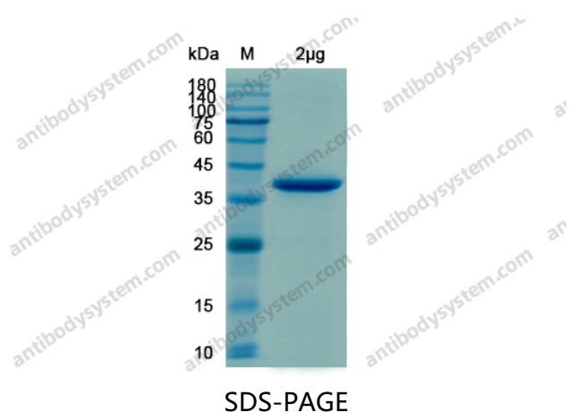
SDS PAGE for recombinant SARS-CoV-2 NSP3 / PL-PRO
