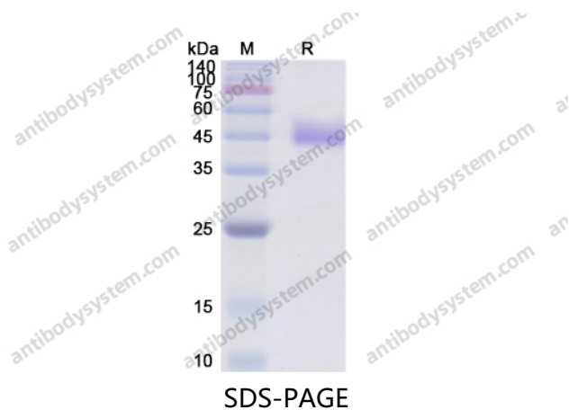
SDS PAGE for recombinant Human CD278 / ICOS
