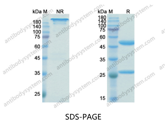
SDS PAGE for Birtamimab
