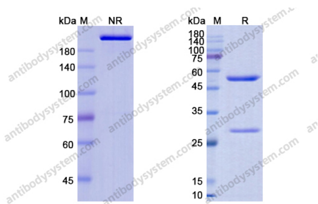
SDS PAGE for HuJ591-Gsmab
