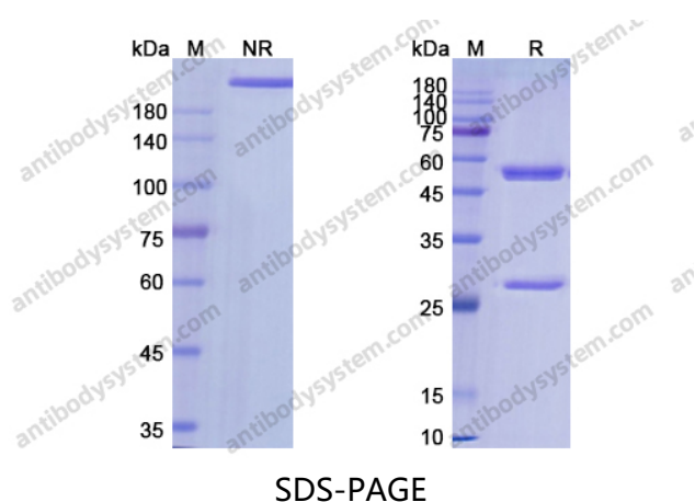
SDS PAGE for Tamrintamab
