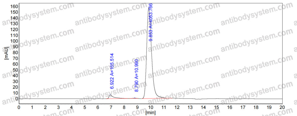
SEC-HPLC
