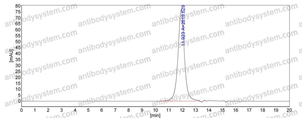
SEC-HPLC
