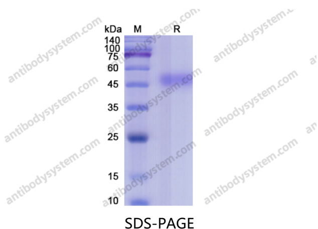
SDS PAGE for recombinant Human CD14
