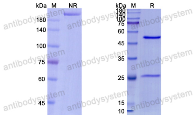
SDS PAGE for Miptenlimab
