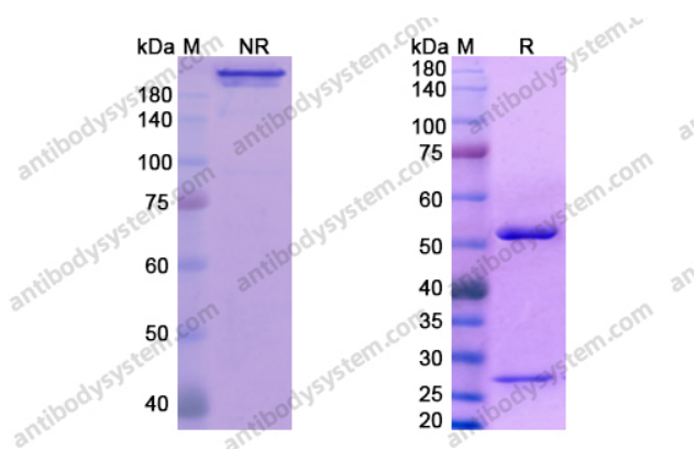
SDS PAGE for Fianlimab
