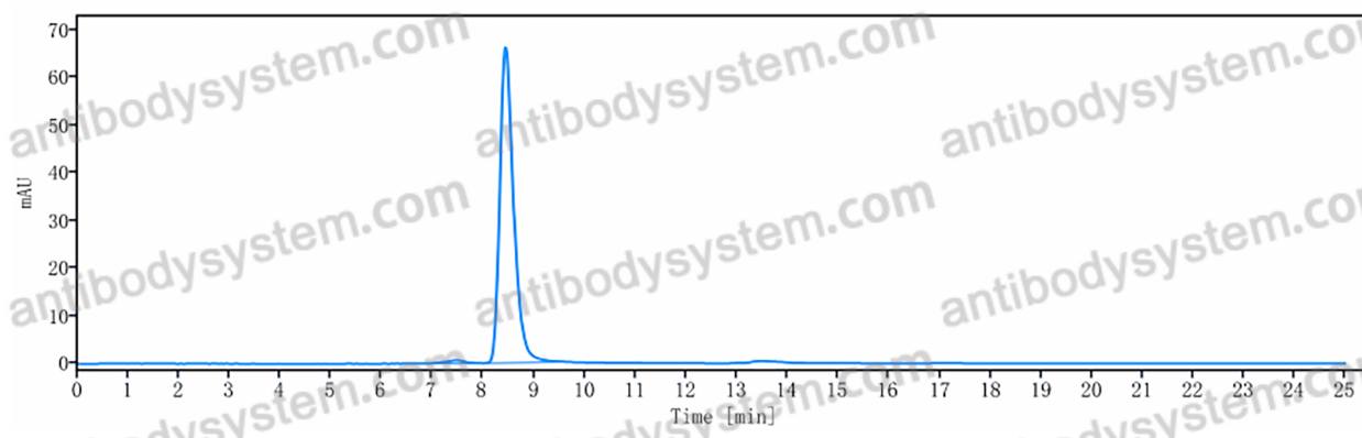
SEC-HPLC
