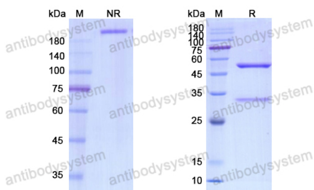
SDS PAGE for Revdofilimab
