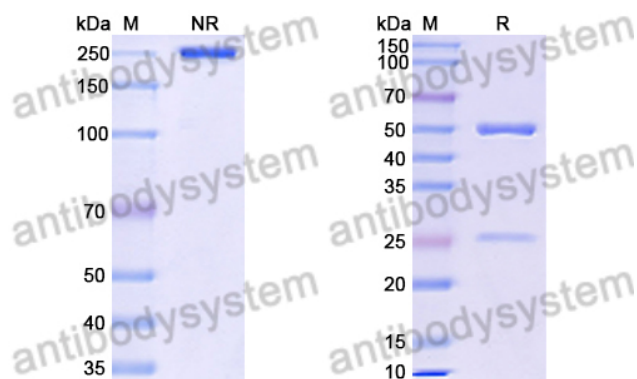
SDS PAGE for DENV-3 Protein prM/prM Antibody
