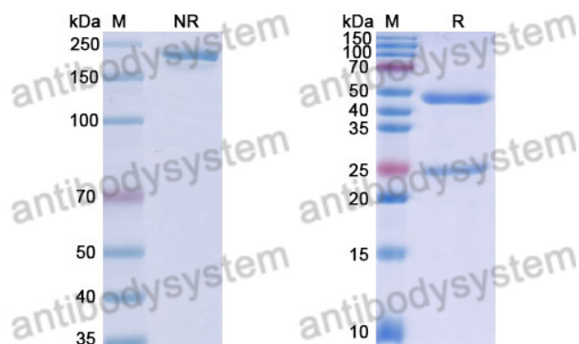
SDS PAGE for DENV-2 Envelope protein E Antibody
