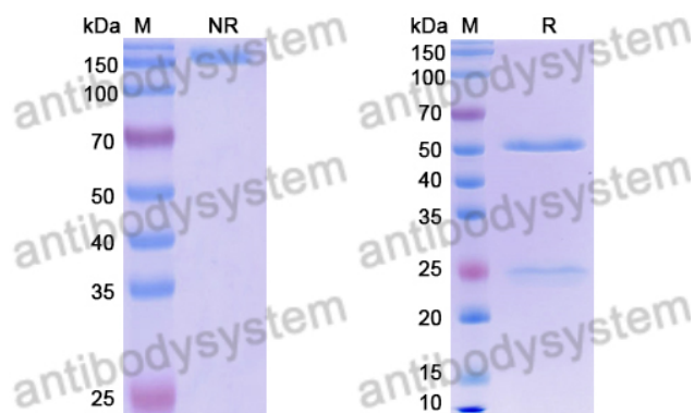
SDS PAGE for DENV-2 Envelope protein E/EDIII A strand Antibody
