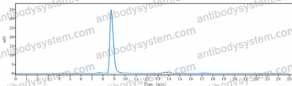
SEC-HPLC
