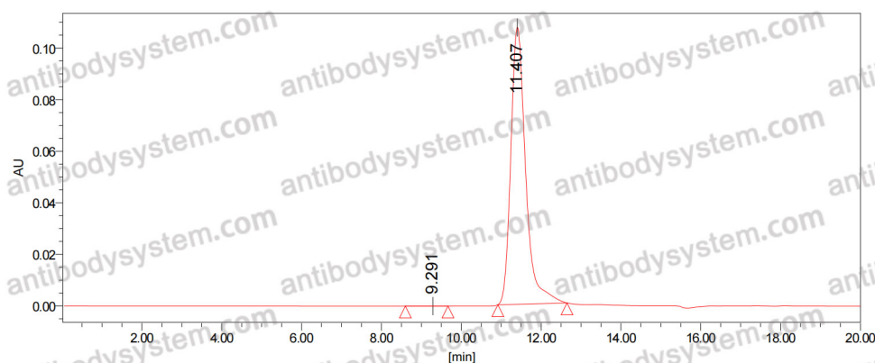
SEC-HPLC
