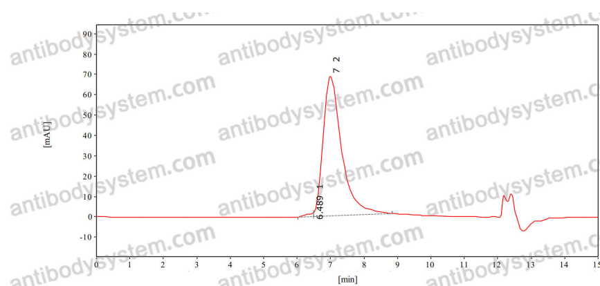
SEC-HPLC
