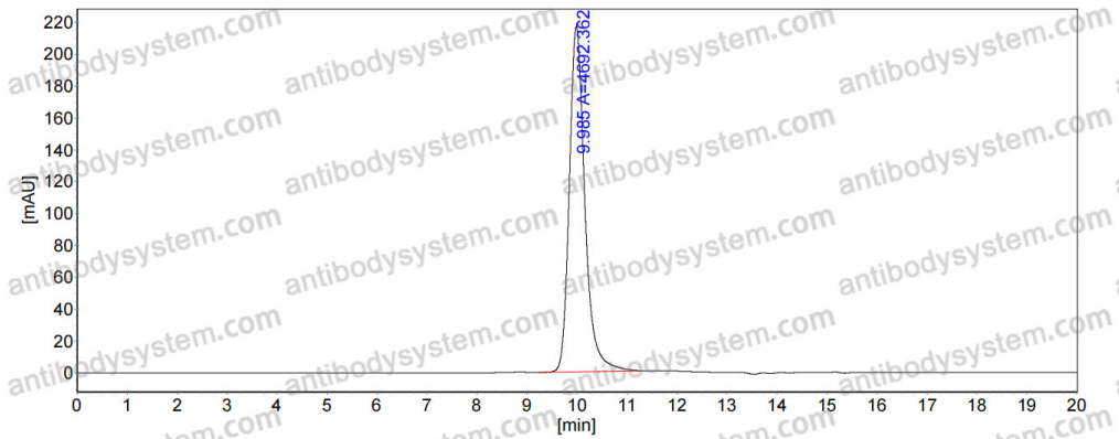
SEC-HPLC
