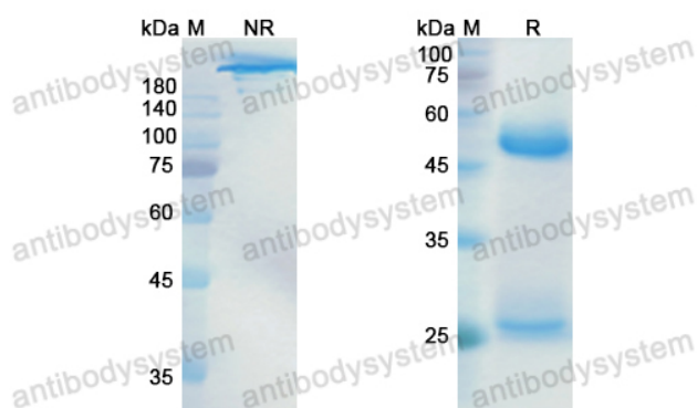
SDS PAGE for Lonigutamab
